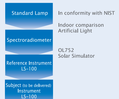
Calibration Flow Chart for LS-100 of Spectroradiometer
